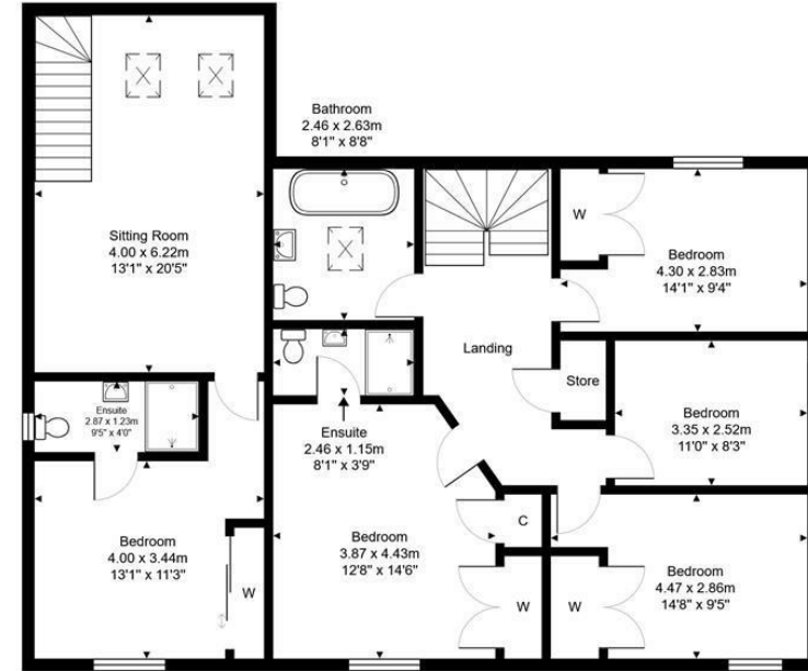
1st Floor
