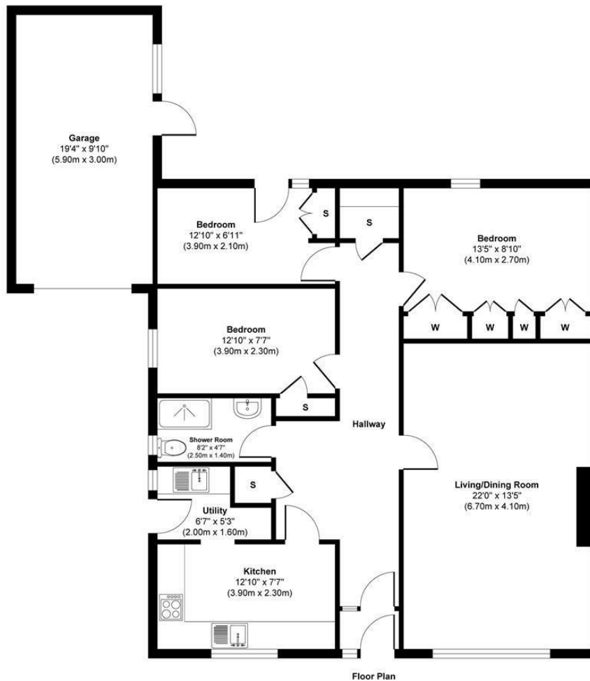
Floor Plan
